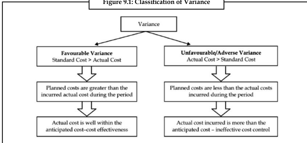
Figure 9.1: Classification of Variance
